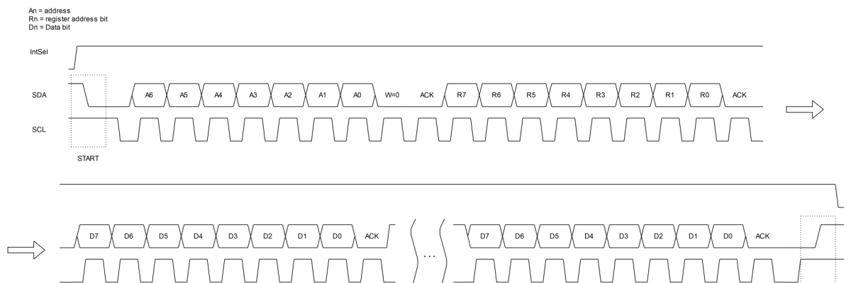
I 2 C write diagram
